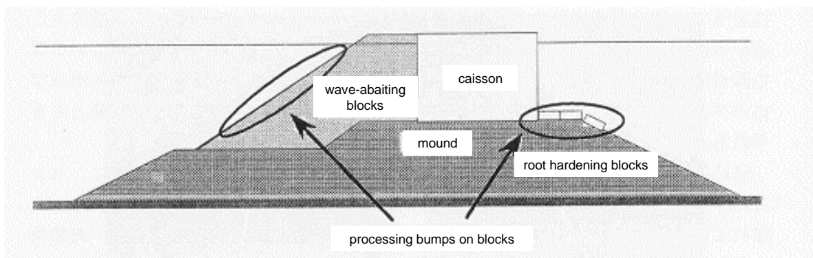
Fig. 3-12. Breakwater areas with irregularities for coral substrates (Harbor & Marine Environment Laboratory 1999)
