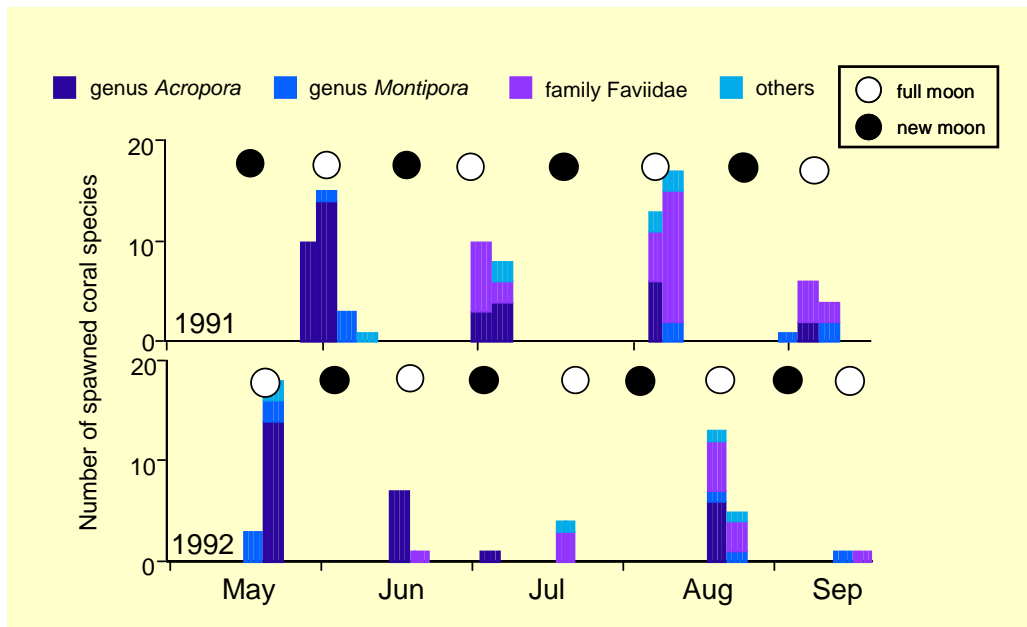
Fig. 3-1 . Pattern of coral spawning at the Akajima Island, Kerama Archipelago (Shows the number of coral species spawned in each of flood tide, middle tide and neap tide)
