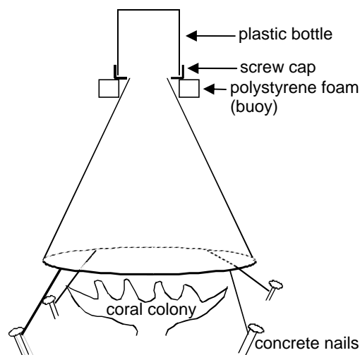
Fig. 3-2 . Schematic view of bundle collector
