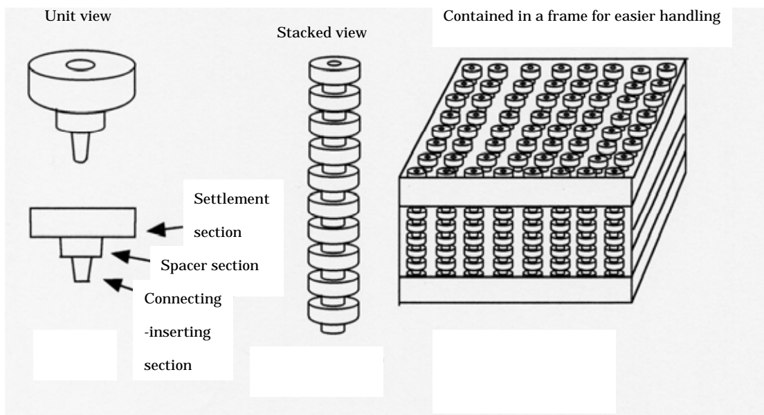
Fig. 6-3 . Coral settlement device and assembling method
