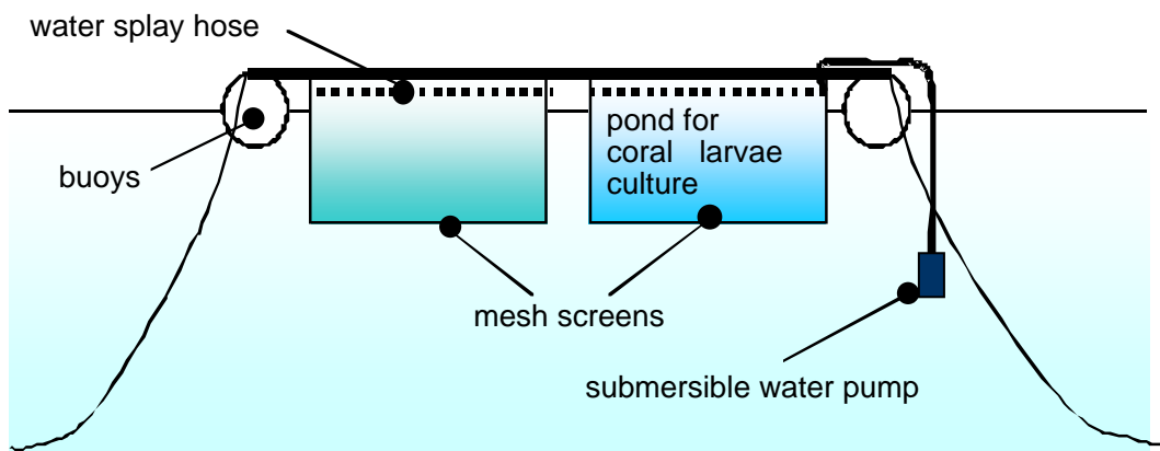
Fig. 3-7 . Large-scale rearing of coral larvae using floating pond
