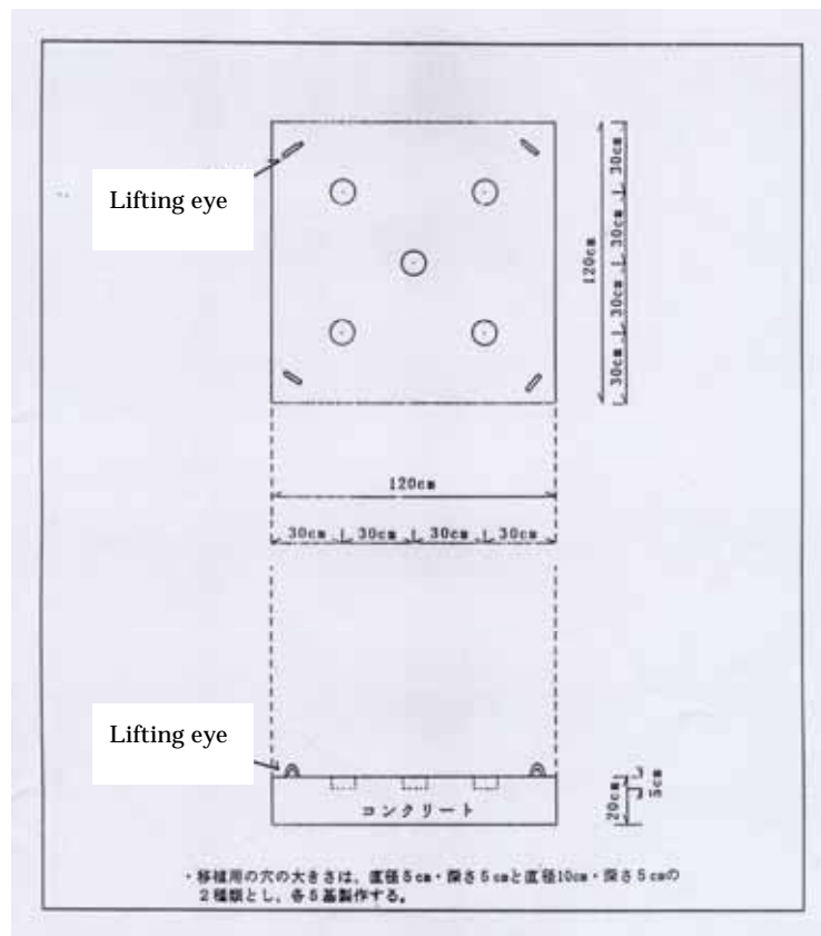
Fig. 6-15 . Dimensions of concrete substrate
