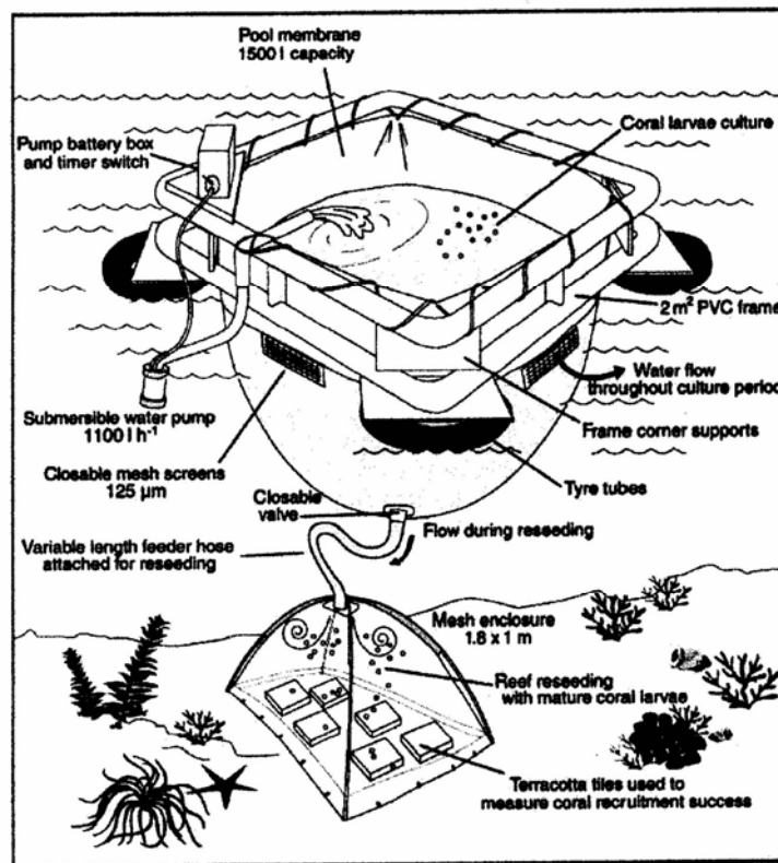
Fig. 3-10 . An example of a method that induces larvae to the tent on the sea bottom from a floating pond (Heyward et al. 2002)
