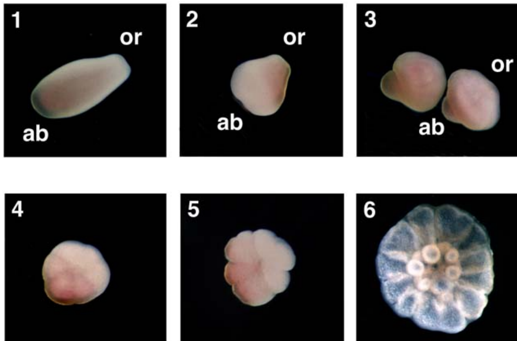
Fig. 3-8 . The process of settlement metamorphosis induced with neuro-peptide
