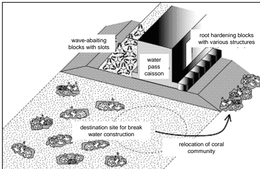
Fig. 5-6 . Schematic view of environmental breakwater at Hirara Harbor (Ishii et al. 2001)
