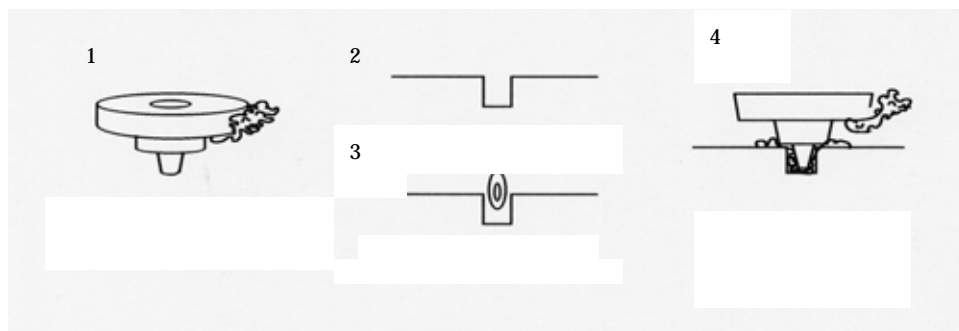
Fig. 6-5 . Settlement device inserting and adhering procedure
