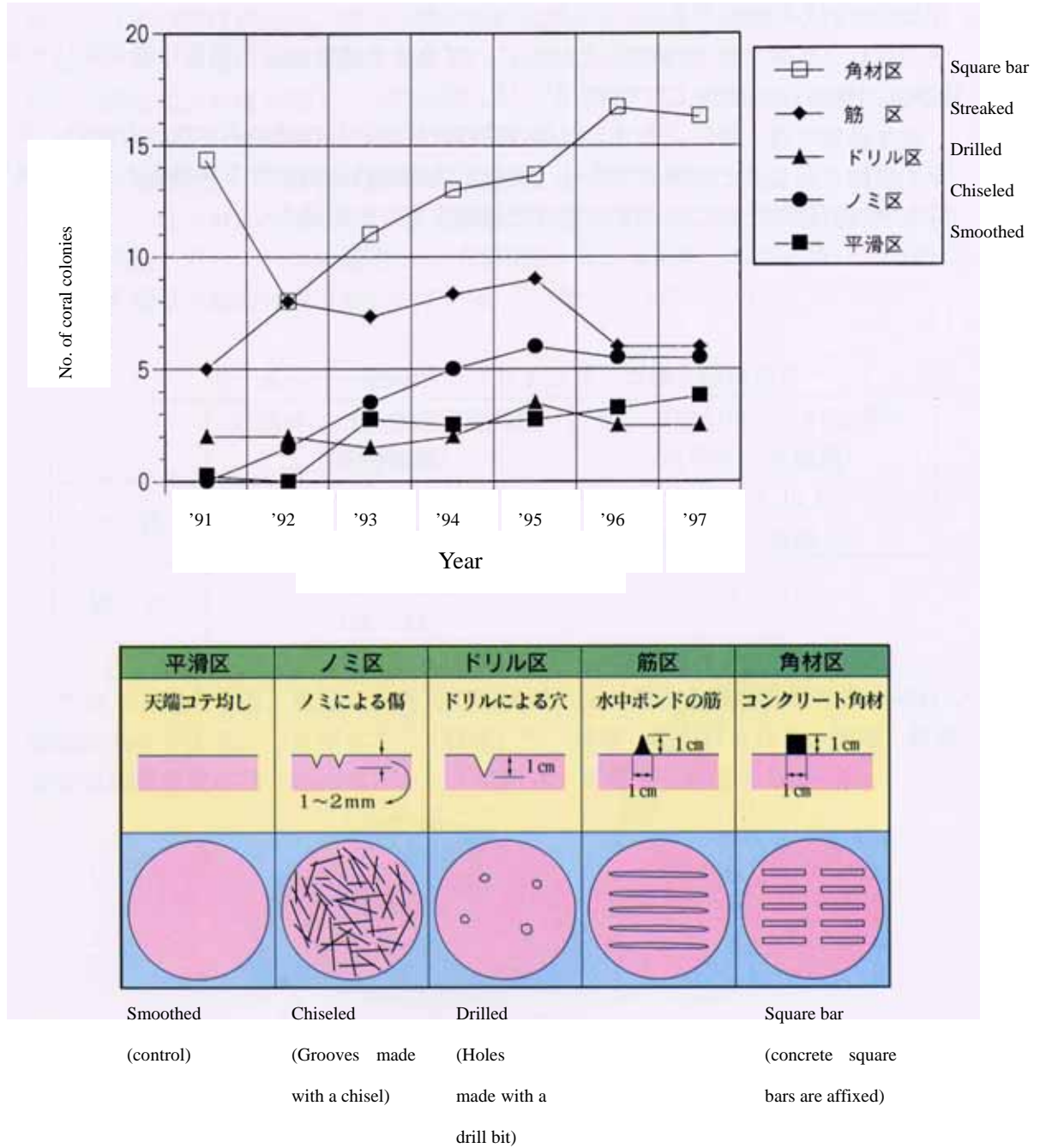
Fig. 3-13. State of settlement of corals at the processed areas of substrate (Harbor & Marine Environment Laboratory 1999)
