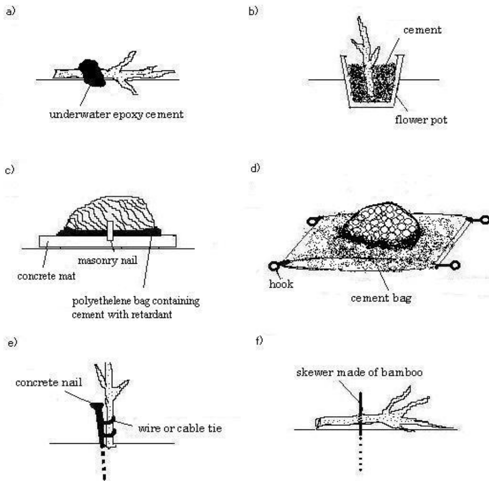
Fig. 4-1 Method of fastening coral fragments
